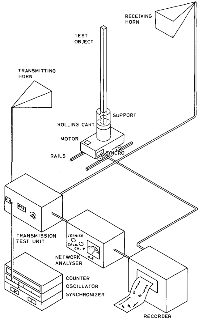
Fig. 2. Experimental setup.
