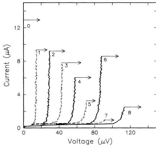
FIG. 2. Current vs voltage for various numbers of solitons at 4.2 K. Full curves: no solitons trapped. Dashed curves: one trapped soliton. The number next to each curve is the total number of solitons and antisolitons moving to produce that curve. The right-pointing arrows at the top of each curve mark the points at which the junction switches out of the various soliton branches. Junction parameters are J=67 A/cm 2 , \lambda_j=59 \mu m, L=875 \mu m, L/\lambda_j=14.8 , \alpha=0.018 , and \beta=0.01 .
