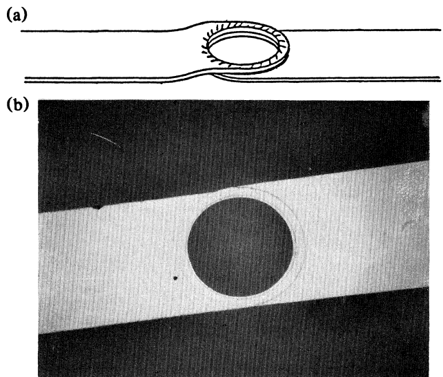
FIG. 1. (a) A schematic of the annular junction that has successfully trapped a single sine-Gordon soliton. (b) An optical micrograph of a typical junction as fabricated, where the overall diameter of the junction is about 300 \mu\text{m} .
