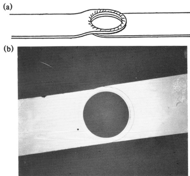
FIG. 1. (a) A schematic of the annular junction that has successfully trapped a single sine-Gordon soliton. (b) An optical micrograph of a typical junction as fabricated, where the overall diameter of the junction is about 300 \mu\text{m} .
