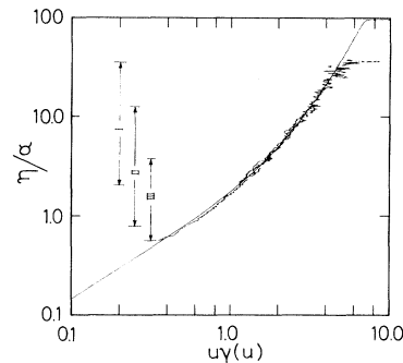
FIG. 4. The universal force-momentum curve for this junction (smooth line) for \beta/\alpha=0.556 . The rough lines are data taken with a single soliton trapped in the junction (on the n=1 step) at three different temperatures, all fitted with the constant \beta/\alpha . Notice that the force ( \eta ) has been scaled with \alpha . The three Roman numerals show the three ranges of \eta/\alpha covered by the three temperatures from 4.2 K, region I, to some intermediate temperature, II, to the highest temperature, about 6.5 K, region III.
