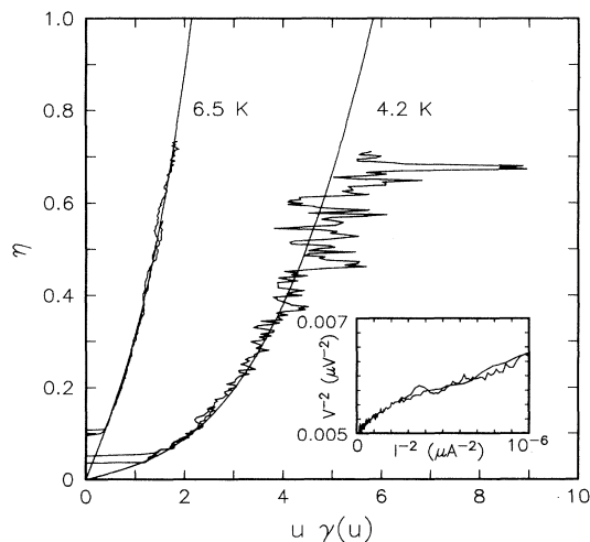
FIG. 3. Force ( \eta ) vs momentum [ u\gamma(u) ] for the n=1 step (a single trapped soliton) for two temperatures. The curve at the left is for a temperature just below T_c , about 6.5 K. It was fitted as described in the text with \beta=0.1 , \alpha=0.18 , V_c=12.51 \mu\text{V} , and I_0=3.46 \text{ mA} . The curve at the right was taken at about 4.2 K and fitted with \beta=0.01 , \alpha=0.018 , V_c=14.38 \mu\text{V} , and I_0=12.7 \text{ mA} .
