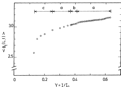
FIG. 4. Calculated third ZFS [ \langle \phi_3(L,t) \rangle vs \gamma ]. The \gamma intervals a – c correspond to soliton configurations shown in Figs. 2(a)–(2c).
