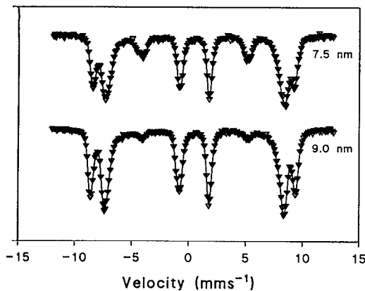
FIG. 4. Mössbauer spectra of 7.5 nm (the upper spectrum) and 9.0 nm maghemite 13 particles in a magnetic field of 4.35 T parallel to the \gamma -ray direction. The spectra were obtained at 5 and 15 K, respectively.
