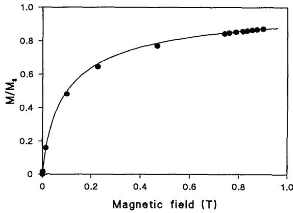
FIG. 1. The magnetization, at room temperature, as a function of applied magnetic field. The full curve is the best fit obtained using the method of Chantrell et al. 14
