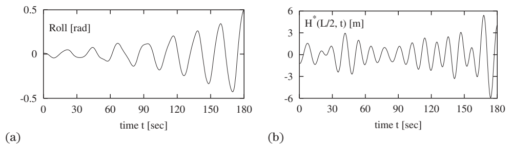
Fig. 10. Most probable roll response (a) and critical wave episode amidships (b). Heading \psi = 60^\circ
