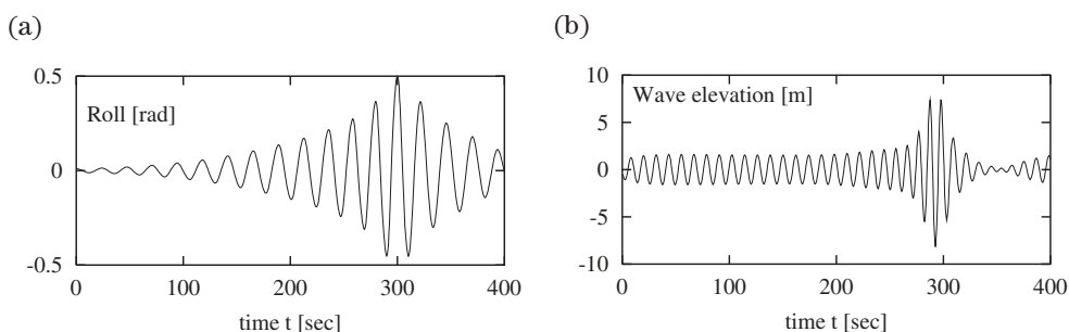
Fig. 3. a Most probable roll response yielding a limiting roll angle of \phi_0 = 0.5 radians at t_0 = 300 s. b Corresponding critical wave episode amidships
