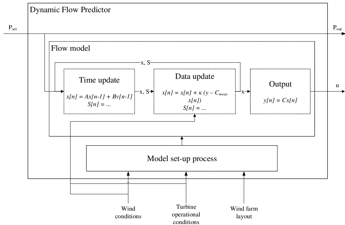
Figure 1. System structure of a dynamic flow predictor (DFP), showing the system update process and Kalman filter time update and data update.
