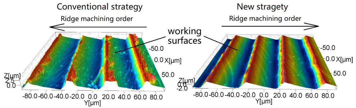
Figure 1: The geometries obtained by applying the two micro milling strategies, scanned by a confocal Laser 3D scanner (Olympus Lext): (left) micro features by the conventional milling strategy with burrs formed on the edges and (right) the burr-free features by the new milling strategy.
