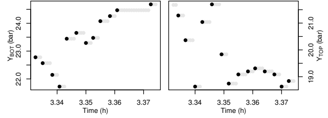
Fig. 2. Observations of the training set, left column show the bottom pressure while right column show the top pressure. grey dots indicate the provided data set while black dots indicate the data used for estimation. described by a Gaussian random variable i.e.
