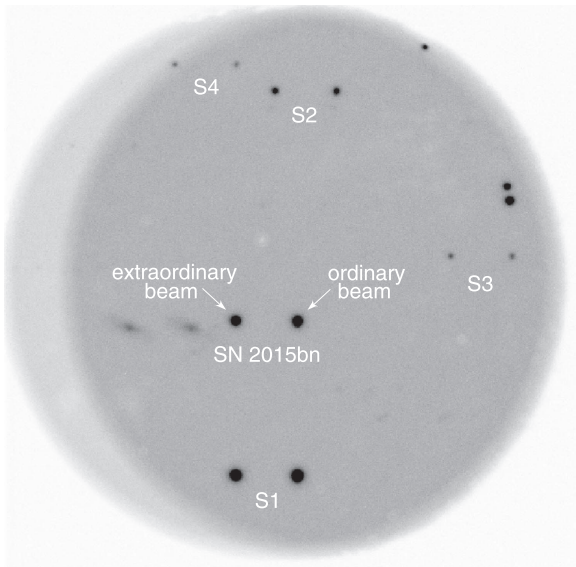
Figure 1. SN 2015bn observed with NOT+ALFOSC in polarimetric mode on 2015 March 16, close to maximum light. Each object appears twice on the image with a separation of 15'' . There are four more point-like sources (marked S1–S4) for which both the ordinary and the extraordinary image appear in the FOV. S1 has an adequate S/N and was used for the determination of the Galactic ISP.
