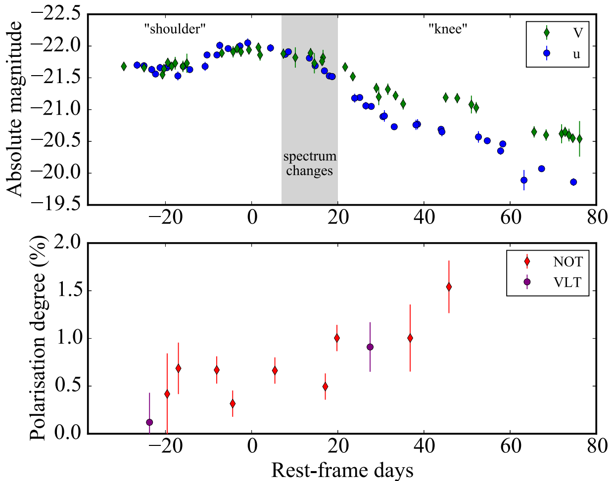
Figure 3. Different stages in the evolution of SN 2015bn. In the upper panel, we plot the ultraviolet and visual absolute light curves from Nicholl et al. (2016b) and we mark the two major undulations in the light curve. The shaded region highlights the time interval where changes occurred in the optical spectrum (Nicholl et al. 2016b). The lower panel shows the simultaneous evolution of the polarization degree from our V-band imaging polarimetry (red). In addition, we show the integrated V-band polarization from the two epochs of VLT spectropolarimetry (purple; Inserra et al. 2016). The data obtained from day +20 and onward show a statistically significant increase in polarization.
