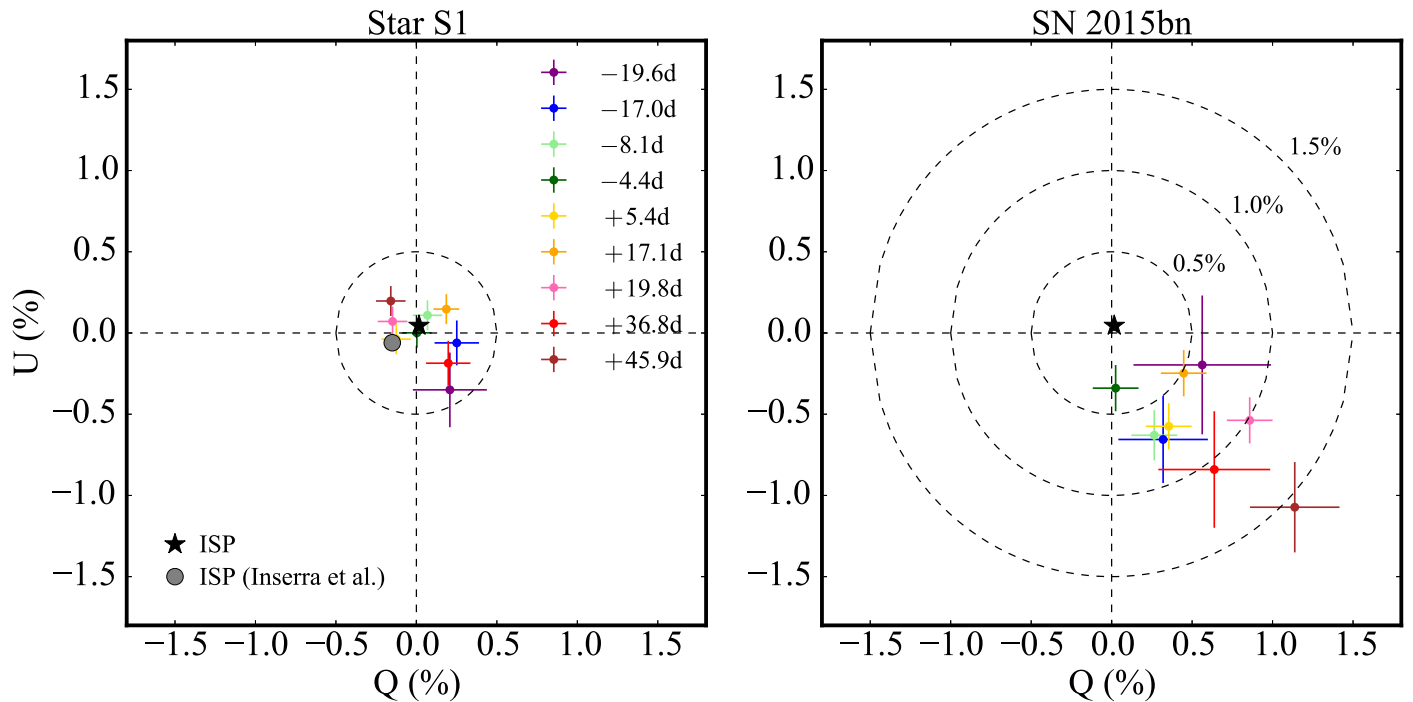
Figure 2. Stokes Q - U plane for star S1 (left) and SN 2015bn (right). The different epochs are color coded as indicated. The black star shows the location of the ISP as determined by S1. For comparison, the ISP estimate by Inserra et al. (2016) is also shown. In both cases, the ISP is found negligible. The SN data on the right panel have been corrected for the ISP. Concentric circles of equal polarization have been drawn to guide the eye. The last three measurements indicate an increase in the SN polarization with time.
