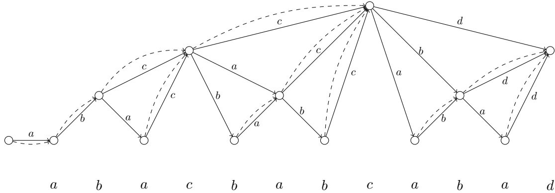
Figure 2: The level automaton constructed from the string abacbabcabad .
