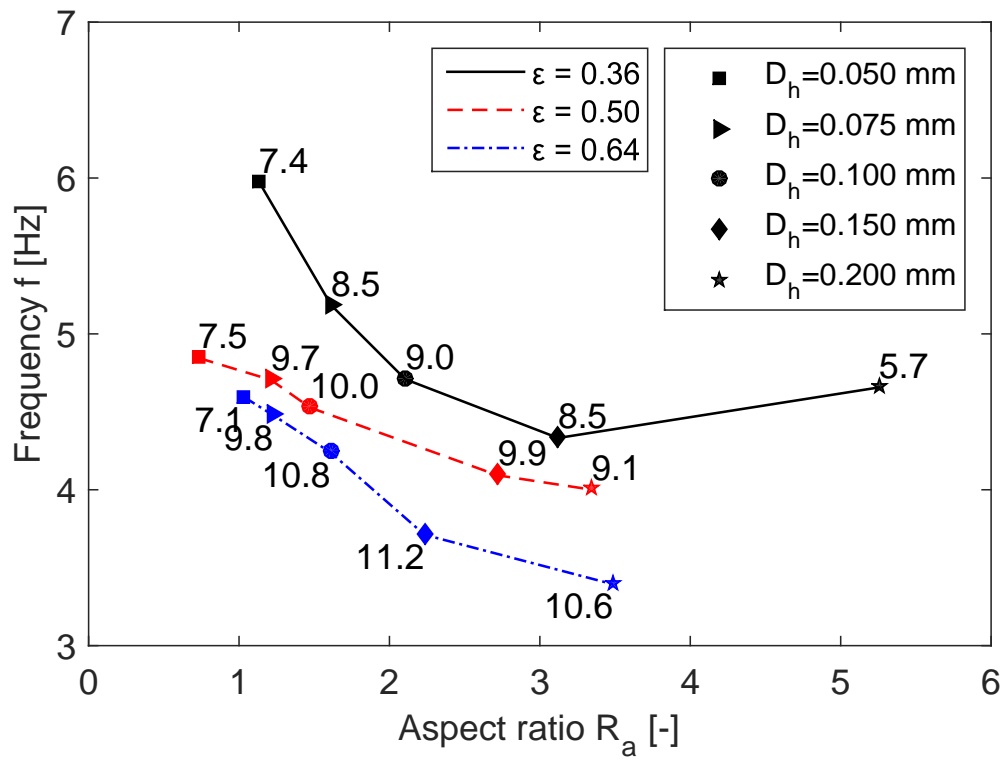
Figure 8: Optimum frequency f and aspect ratio R_a for regenerators using parallel plate matrix under different hydraulic diameters D_h and porosities \epsilon
