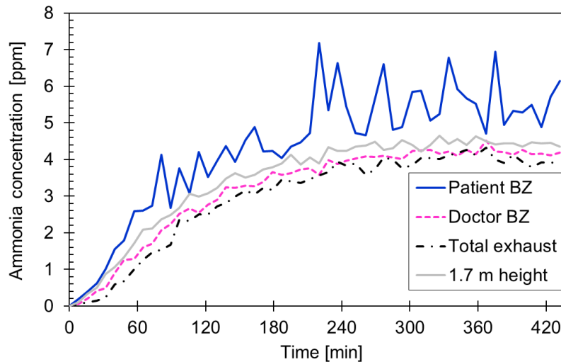
Fig. 6. Ammonia concentration in the sampling points throughout the chamber for the exposure period (7 hours 20 min) during the condition of ‘1.6 ACH’ (reference case).
