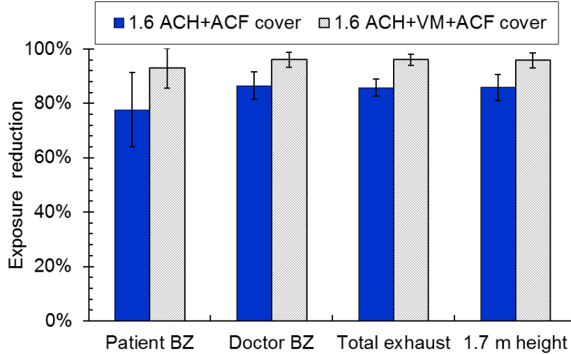
Fig. 8. Exposure reduction using the ACF as a blanket and when using the VM combined with ACF as a cover compared to the case of background mixing ventilation alone.
