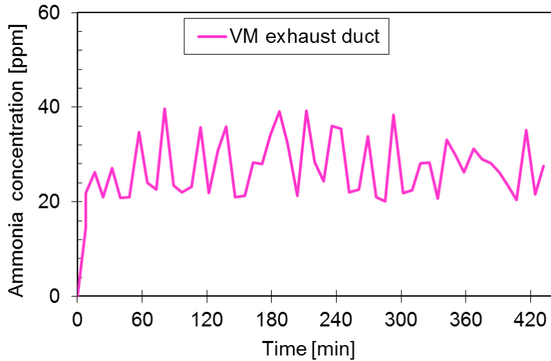
Fig. 9. Ammonia gas concentration measured in the exhaust duct of the VM when there was no ACF material installed.
