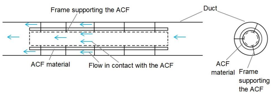
Fig. 4. Diagrammatic representation of the duct ACF material installed inside the exhaust duct connected to the VM.
