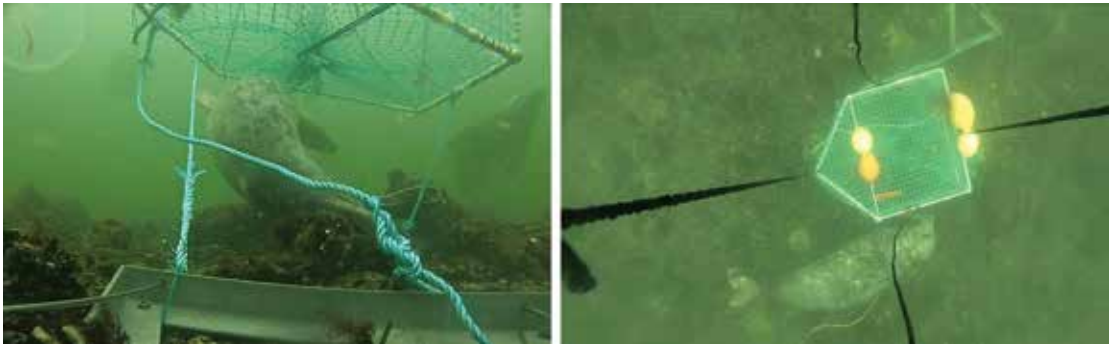
Figure 4: Left: view from the side camera. Right: view from the camera above the cod pot.
