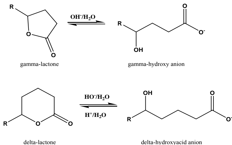
17 Figure III.1. Equilibrium of gamma- and delta-lactone and hydroxycarboxylate anion
