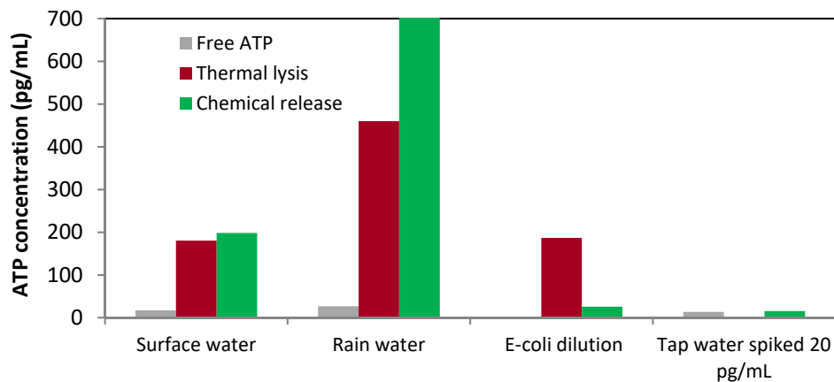
Figure 3. ATP released from the cells by chemical and thermal methods in different types of water. Free ATP is the ATP measured without any releasing step.
