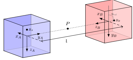
(a) Hydrostatic Test Configuration: Vehicle B is rotated relative to vehicle A such that axis y_A and z_B coincide.
