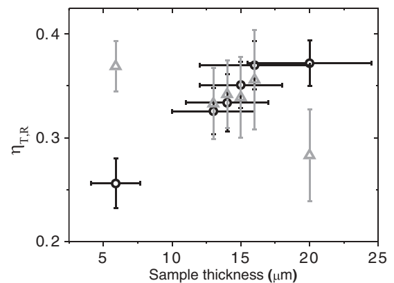
FIG. 4. Overall collection efficiency for each sample thickness as measured in transmission ( \eta_T , gray triangles) and reflection ( \eta_R , black circles). The error bars on the sample thickness are included only on the reflection data.
