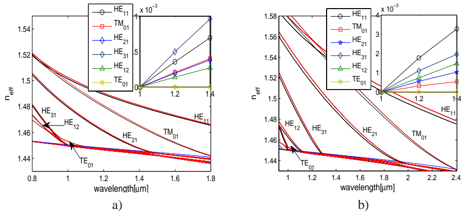
Fig. 11. Effective index plots for K_3/K_1 = 1 (black, lower) and K_3/K_1 = 1.4 (red, upper) for a) 45^{\circ} boundary alignment and b) 90^{\circ} boundary alignment. The insets show the effective index change of the y-polarizations of the modes depending on K_3/K_1 .
