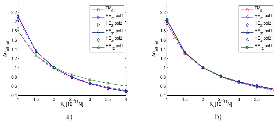
Fig. 13. Relative effective index shift depending on K_1 when applying an external bias for a) 45^\circ and b) 90^\circ boundary alignment. The relative values are taken with respect to the reference configuration. The crossed lines show the fitting curves from the alignment simulations. The plots show the results for K_3/K_1 = 1
