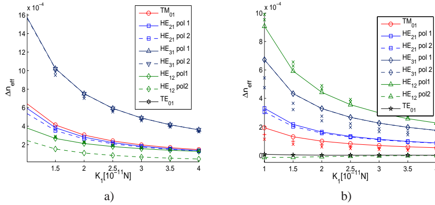
Fig. 12. Relative effective index shift depending on K_1 when applying an external bias for a) 45^\circ and b) 90^\circ boundary alignment. The plots show the results for K_3/K_1 = 1
