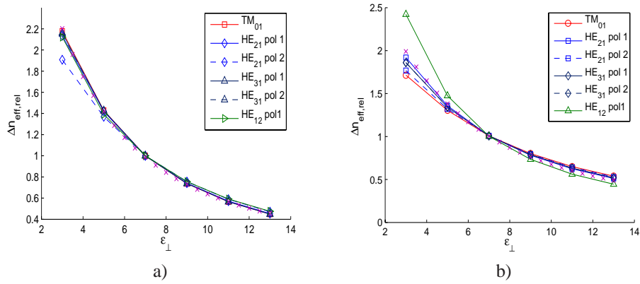
Fig. 10. Relative effective index shift depending on \epsilon_{\perp} for a) 45^{\circ} and b) 90^{\circ} boundary alignment. The relative values are taken with respect to the reference configuration. The crossed lines show the fitting curves from the alignment simulations.
