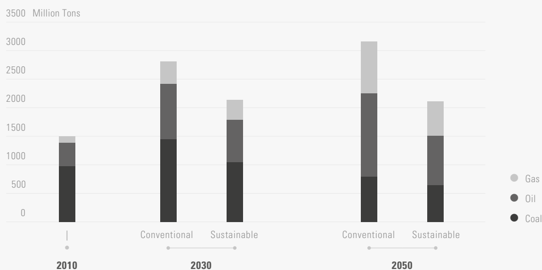
Figure 3.5: CO 2 Emissions
