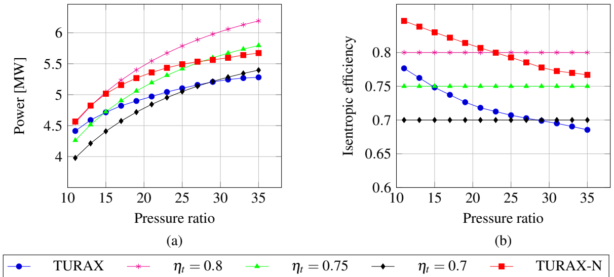
Figure 8: Single exhaust gas configuration. 8(a) Net power output versus pressure ratio and 8(b) Total-to-total turbine isentropic efficiency versus pressure ratio.
