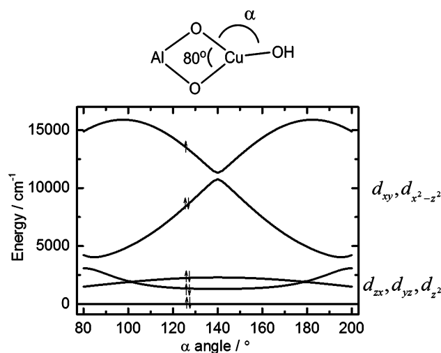
Figure 6. Top: Planar three-coordinate calculated by DFT. 36 Bottom: d-orbital energies are plotted as a function of the O–Cu–OH angle (Walsh diagram) for an angle between 80 and 200°. Energies of the five d orbitals are calculated using Ligfield. 51 The AOM parameters of all three oxygen donor ligands are assumed to be e_\sigma = 7500 cm -1 and e_\pi = 1700 cm -1 . The d orbital with the lowest energy is shifted to zero. The energies of the d–d transitions in this d 9 system can be obtained from the diagram by calculating the energy difference between the d orbital with the highest energy and one of the other four, compared to the energy scale in Figure 5 (right).
