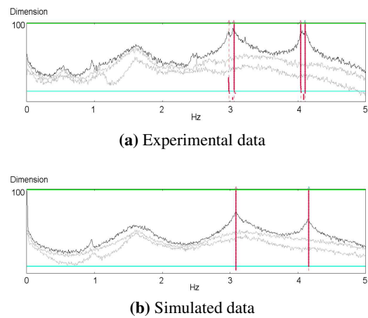
Figure 7: Edgewise modes at \Omega_{low}
