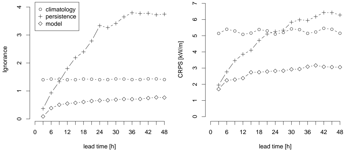
Figure 3: Probabilistic forecast skill as a function of the lead time at Diamond Shoals, as evaluated with both the CRPS and the Ignorance score. The two benchmarks considered are persistence and climatology.
