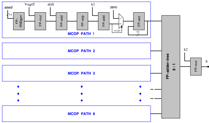
Fig. 3. ASP for 8-path MCOP accelerator.
