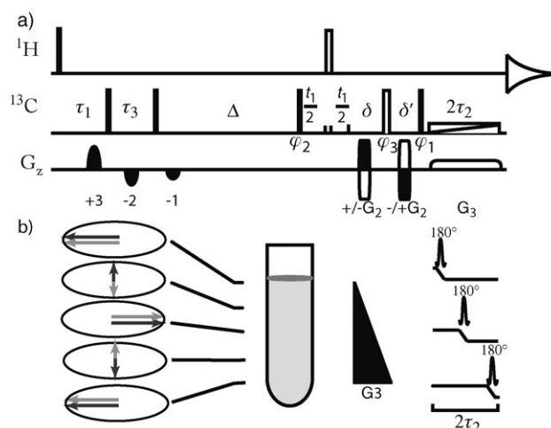
Figure 1. Pulse sequence for the clean HMBC experiment with an initial second-order and terminal adiabatic low-pass J filter. Recommended delays for the filters are \tau_1 = 1/2 [^1J^{\min} + 0.07 (^1J^{\max} - ^1J^{\min})]^{-1} , \tau_2 = (^1J^{\max} + ^1J^{\min})^{-1} and \tau_3 = 1/2 [^1J^{\min} - 0.07 (^1J^{\max} - ^1J^{\min})]^{-1} . [7] \delta and \delta' are gradient delays, where \delta' = \delta + 6 \mu\text{s} accounts for the delay of the first point in the 13 C dimension. The integrals over each gradient pulse G_2 is \gamma_H/2\gamma_C times the integral over gradient G_3 in order to achieve coherence selection. The recommended phase cycle is \phi_1 = \{x, -x, -x, x\} , \phi_2 = \{x, x, 4(-x), x, x\} and \phi_3 = \{4(x), 4(y), 4(-x), 4(-y)\} with the receiver phase \{x, -x\} . The dephasing under one-bond couplings during the adiabatic filter by spatially dependent application of the 180° 13 C pulse is shown in (b).
