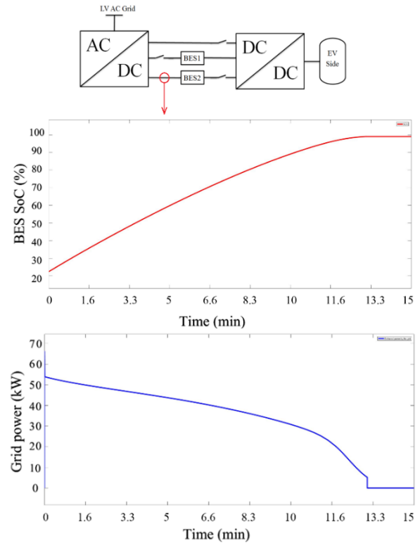
Figure 8. Active power delivered by the LV grid
